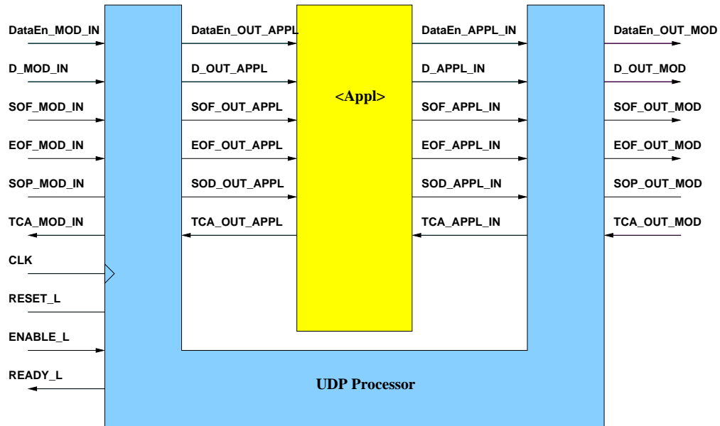
Figure 19: UDP Processor Interface
