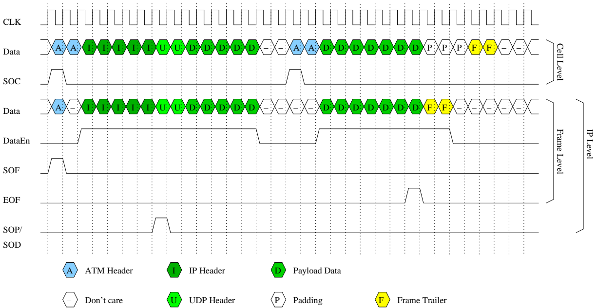
Figure 20: Timing diagram for different signalling protocols
