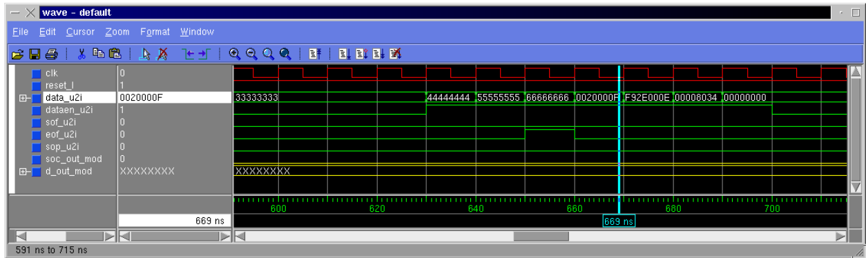
Figure 14: Simulation input coming from a UDP based application
