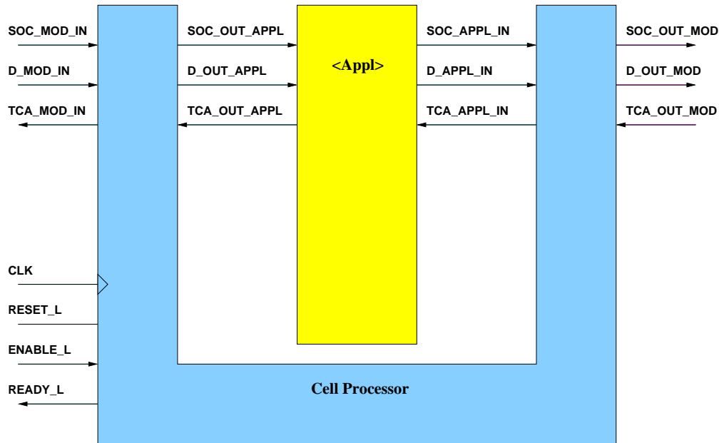
Figure 16: Cell Processor Interface
