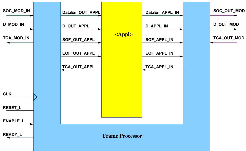
Figure 17: Frame Processor Interface
