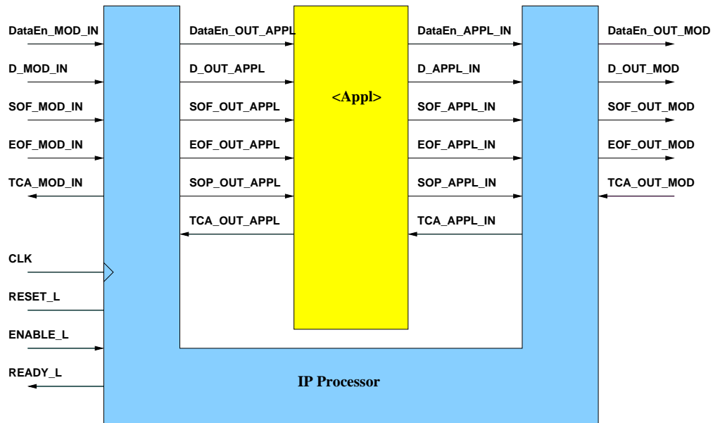
Figure 18: IP Processor Interface
