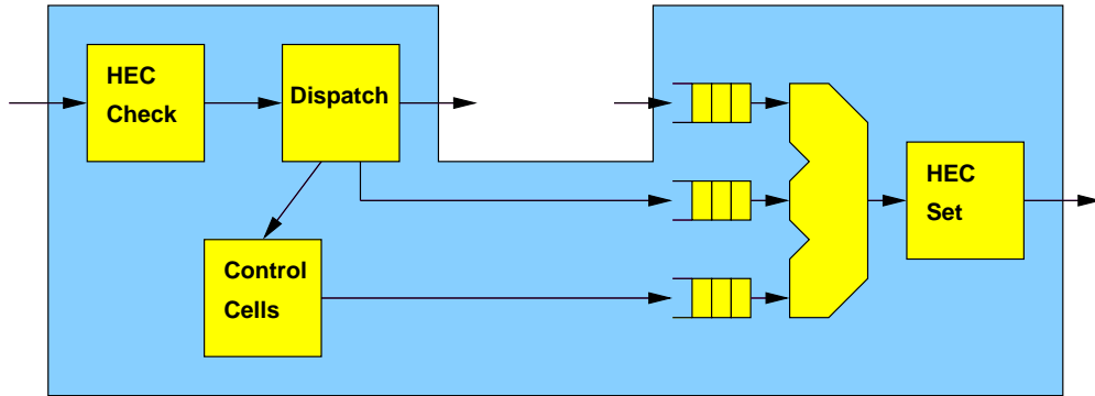
Figure 5: Cell processor
