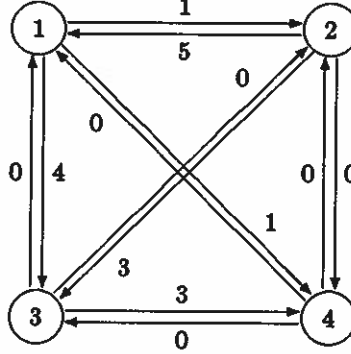
Figure 1: Example of transformation from SCS to LPP ( S = \{cbadef, fcbade, adefcd, fcadfb\} )
