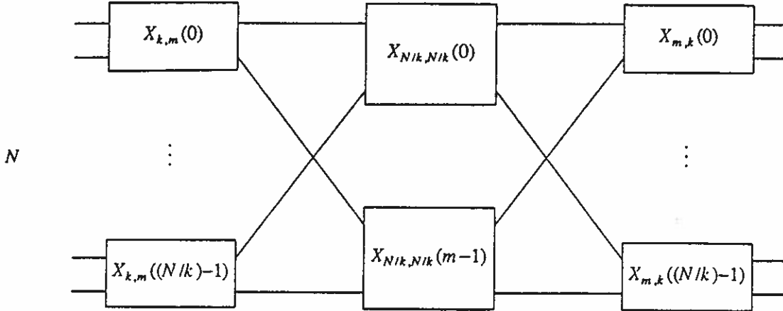
Figure 1: Clos Network
