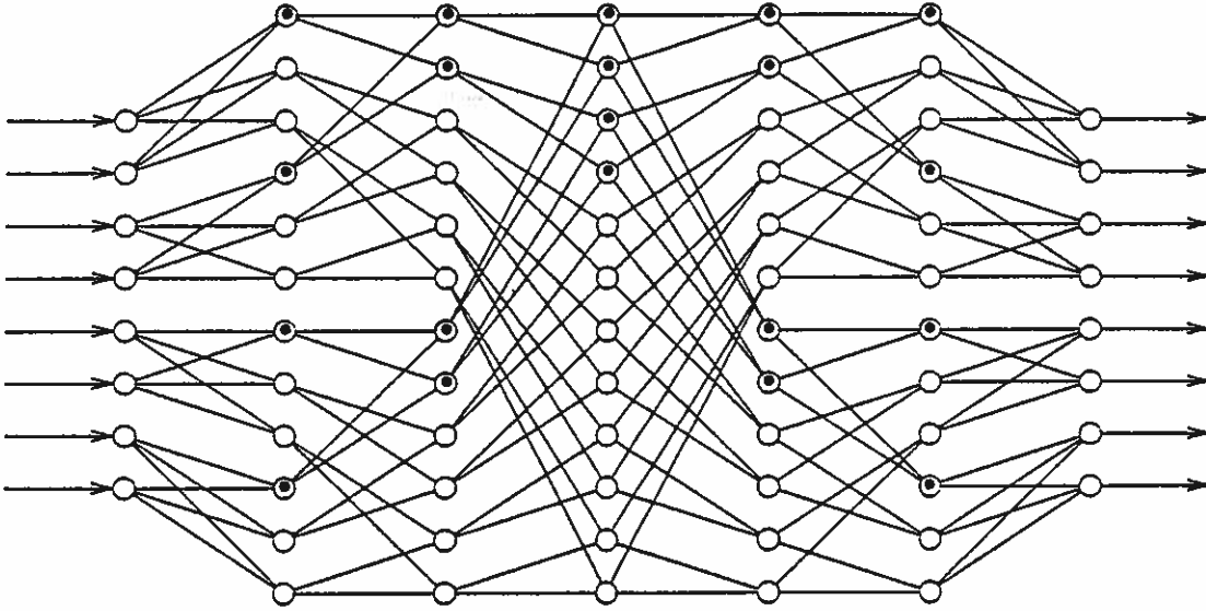
Figure 3: Cantor Network
