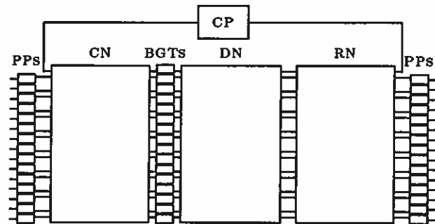
Figure 1: One-to-Many Connection
