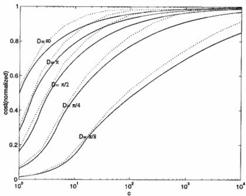
Figure 1: Lowerbound as calculated from Eqn. 3, compared with simulation on a network with 50 switches. The costs are normalized. Solid lines are calculations, dotted lines are simulations.
