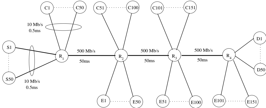
Figure 4: Multi-Hop Path Network Configuration
