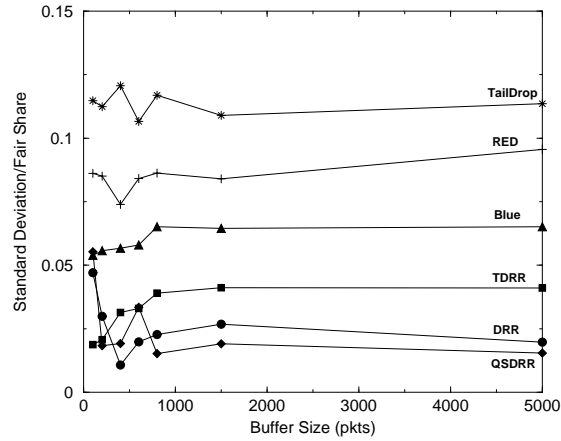
Figure 6: Standard deviation over fair-share for TCP Reno flows over a single-bottleneck link
