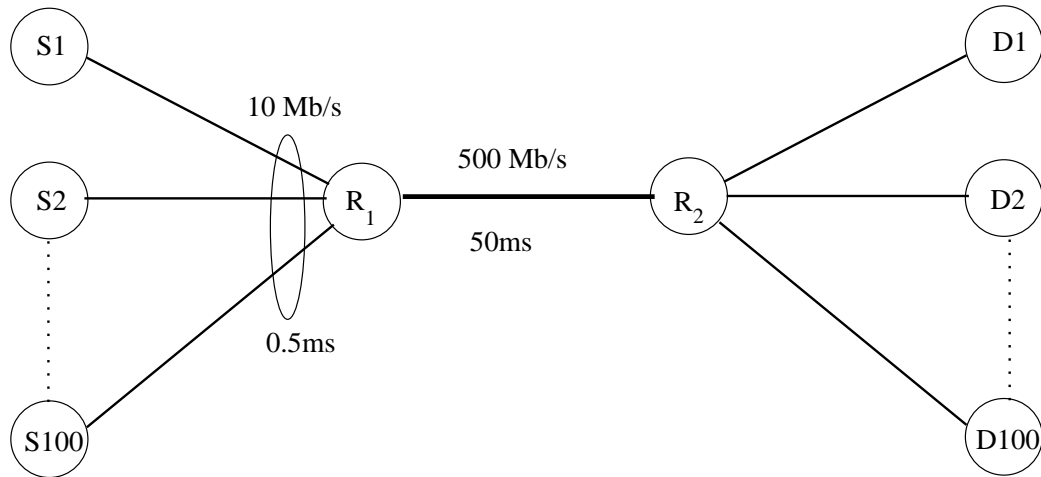
Figure 2: Single Bottleneck Link Network Configuration
